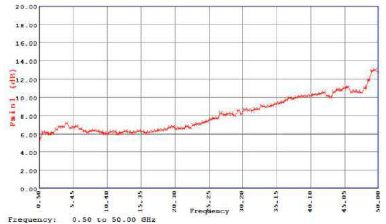
Figure 4. Typical Noise Receiver Calibration Using MT7553B03
