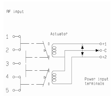
WITH SUPPRESSION DIODES R585-7-030/R585-7-230/R585-7-430
