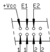
Solder pins
