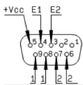
D-Sub connector
