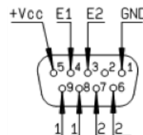
D-Sub connector
