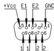
D-Sub connector
