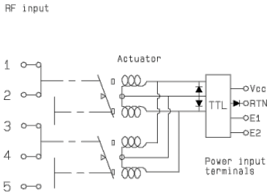
WITH CUT-OFF (SUPPRESSION DIODES ARE INCLUDED) R585-5-000/R585-5-200/R585-5-400
