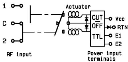
WITH CUT-OFF & TTL DRIVER (SUPPRESSION DIODES ARE INCLUDED) R570-5-100
