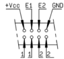
Solder pins
