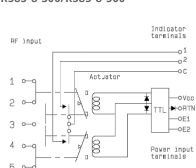
WITH TTL DRIVER & INDICATOR CONTACT (SUPPRESSION DIODES ARE INCLUDED) R585-8-100/R585-8-300/R585-8-500
