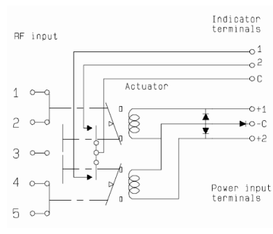
WITH SUPPRESSION DIODES & INDICATOR CONTACT R585-8-030/R585-8-230/R585-8-430
