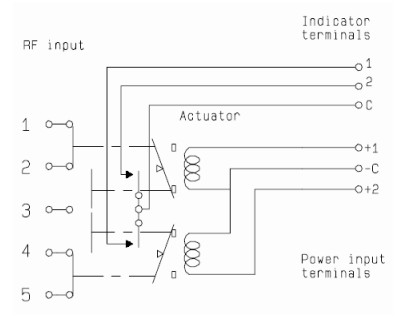
WITH INDICATOR CONTACT R585-8-000/R585-8-200/R585-8-400
