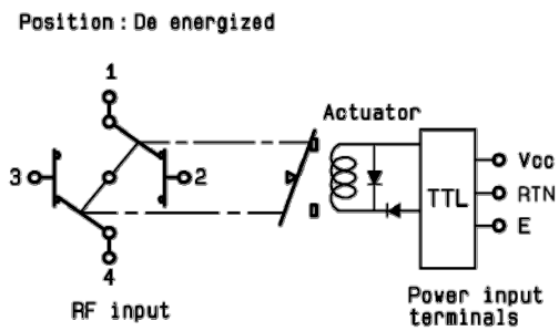
WITH TTL DRIVER (SUPPRESSION DIODES ARE INCLUDED) R577-1-100
