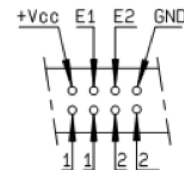
Solder pins
