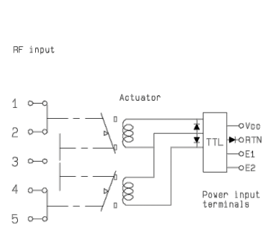
WITH TTL DRIVER (SUPPRESSION DIODES ARE INCLUDED) R585-7-100/R585-7-300/R585-7-500
